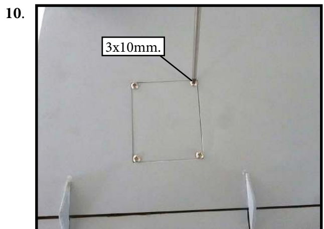
Route the servo lead for the flap servo out at the root of the wing. Connect the flap servo to the radio system. With the radio system on, place the flap servo into position.
