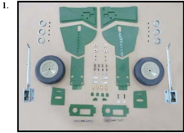
Install retractable landing gear at the Wing.
