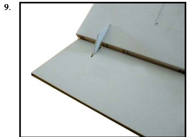
Once adjusted, make sure all clevis retainers are in position. Apply a drop of threadlock near the clevis, then tighten the nut against the clevis to keep the linkage from changing length inside the wing.
