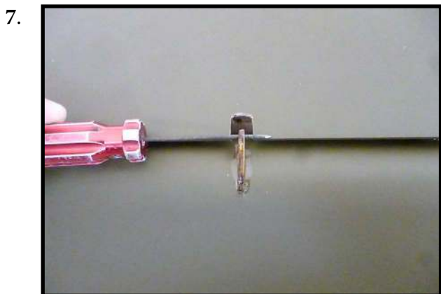
Route the servo lead for the flap servo out at the root of the wing. Connect the flap servo to the radio system. With the radio system on, place the flap servo into position.
